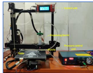
3D-Printer
